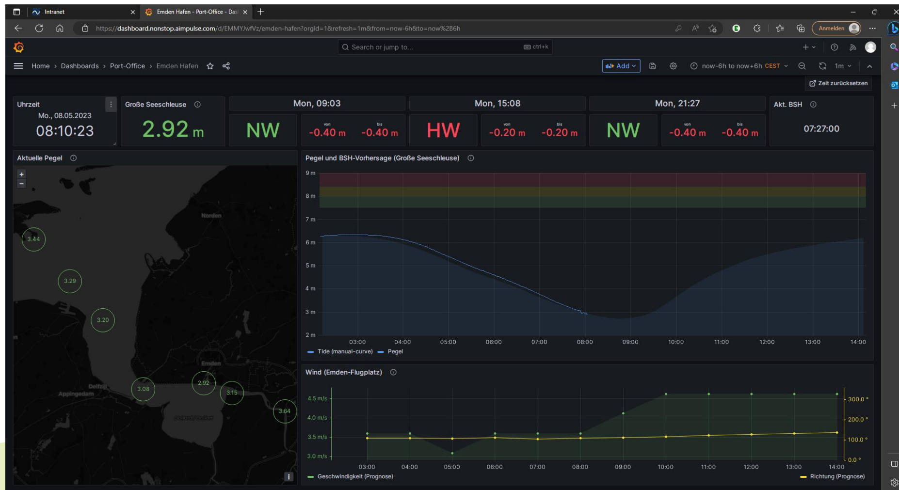
Figure 40. Dashboard created for the Port Office Department, featuring wind conditions, water level measured and predicted values, and customized reference points indicating need for action following a traffic light system.
