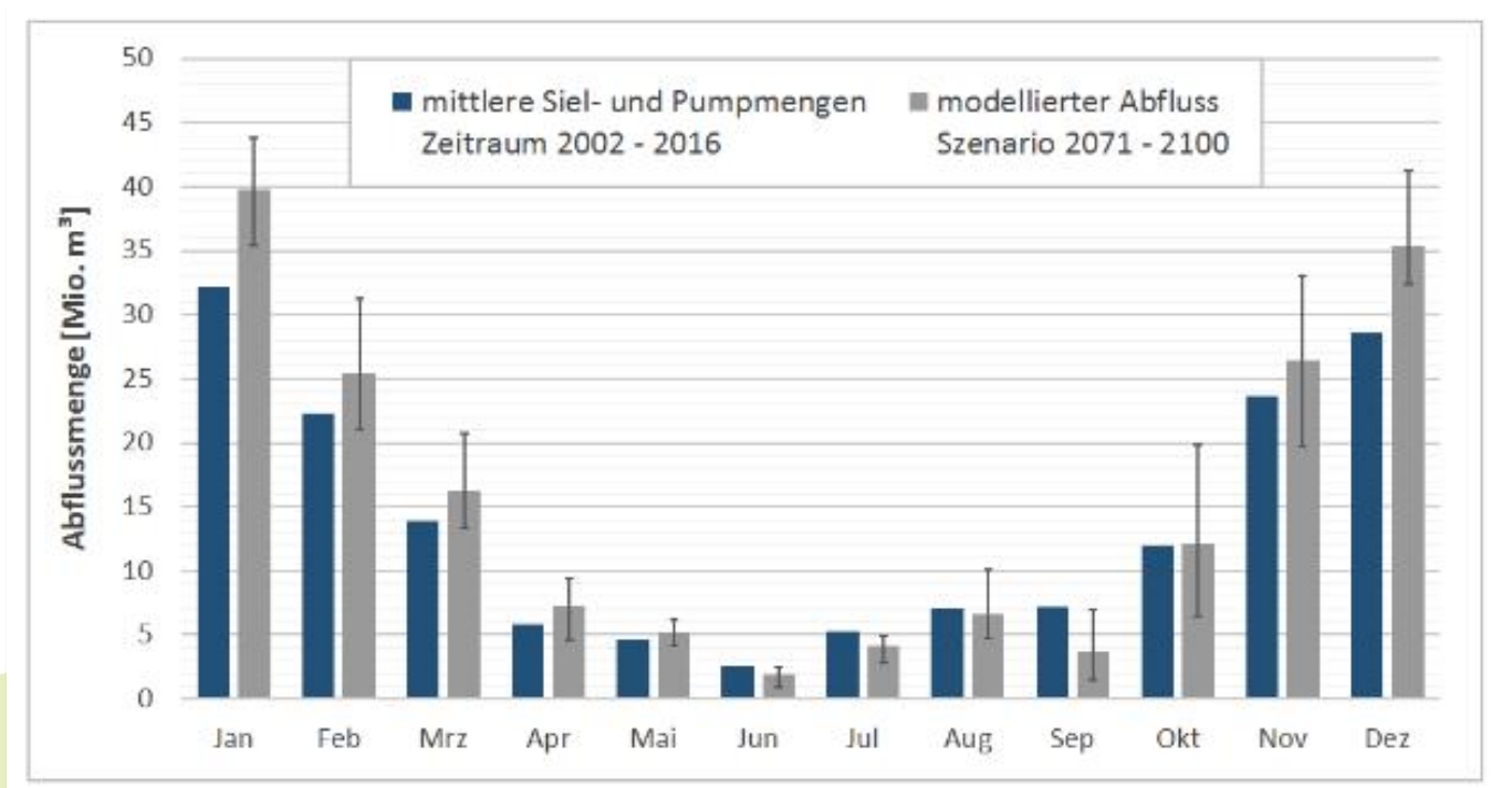
Figure 7. Model based estimation of the seasonal freshwater discharge in the area of the I. Entwässerungsverband due to climate change. Blue: Average of pumped discharge 2002-2016. Grey: average of modelled discharge for different climate scenarios 2071-2100. Source: Spiekermann et al. (2018).
